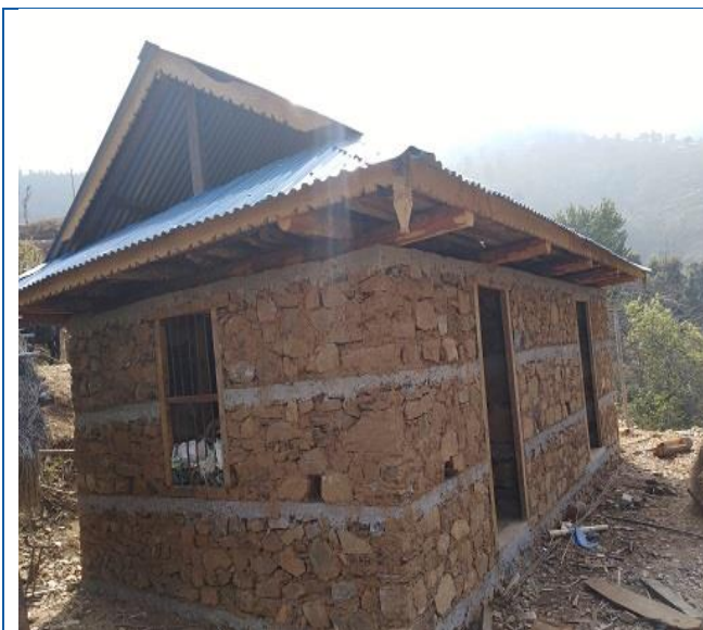
Caption: Stone mud mortar building in Tosharam Khola ward no-07 of Tinpatan Rural Municipality of Sindhuli district. Construction of this house is completed and beneficiary is waiting for government 3 rd tranche.
