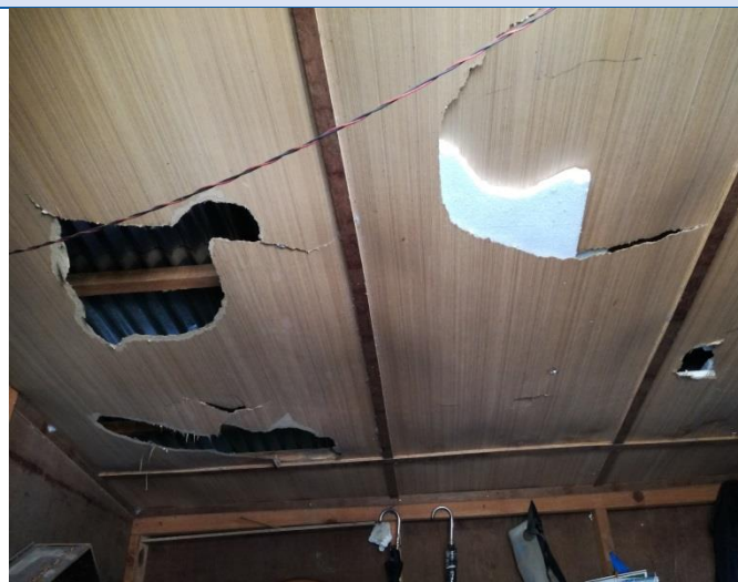
Bungamati Ward no. 22, Lalitpur Metropolitan City, the modification of temporary shelter constructed using wooden frames. The damaged roof has been fixed using the CGI sheets. The beneficiary of the house has received the 1 st tranche.
